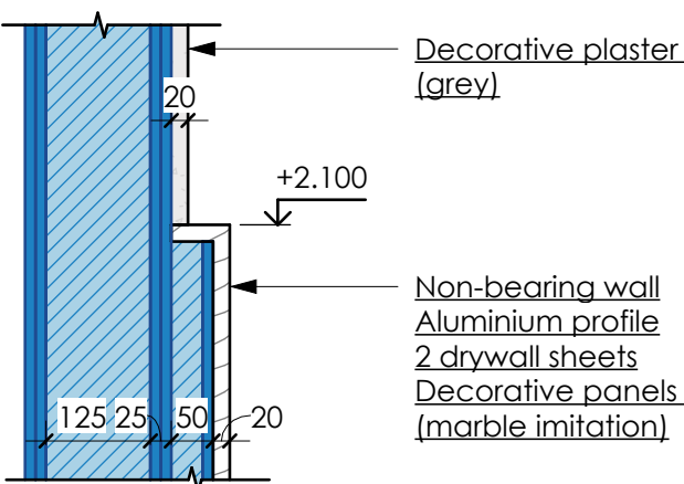
Section 1-1
