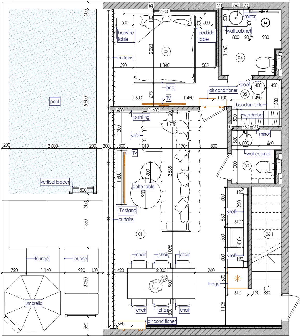
Ground floor
